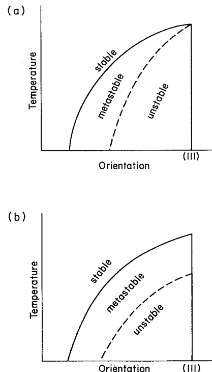
FIG. 2. Si coexistence curve (solid line) and spinodal line (dashed line). (a) Without stress, (b) with stress.
