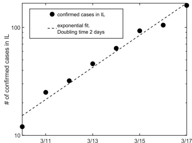
Figure 1 Number of confirmed COVID_19 cases in Illinois vs. date. The vertical axis is a logarithmic scale. The linearity of this graph shows the exponential growth with doubling time of 2 days expected early in an epidemic. The simulation model is calibrated to replicate this trend.
