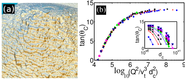
FIG. 3 (color online). Results from simulation of the CA model. (a) Portion of a typical simulated landscape. The figure clearly shows distinct geomorphological regimes or facies, as observed in the field [6]. (b) Critical angle for the contact line formation on a travertine dome, plotted according to Eq. (5), showing data collapse, as predicted by theory. Inset: Raw data.
