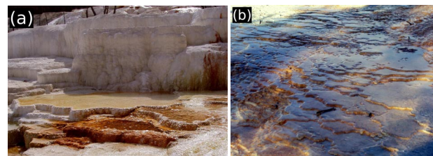
FIG. 1 (color online). Travertine formation at Angel Terrace, Mammoth Hot Springs, WY, USA. (a) A large pond, of order 1 m in diameter, and smaller features. (b) A portion of the flow system about 25 meters from the vent, on the scale of centimeters.
