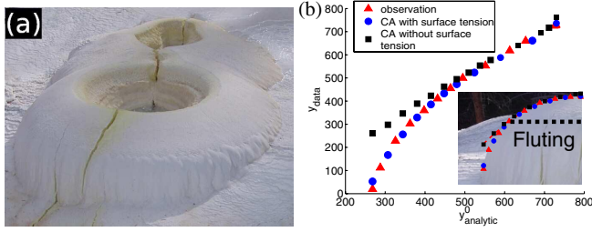
FIG. 2 (color online). Travertine dome at Mammoth Hot Springs, WY, USA. (a) Dome whose central pond is 50.3 cm in diameter. (b) Dome height as a function of \theta . Horizontal axis: Analytical prediction from Eq. (4). Vertical axis: Simulated dome (CA) with no surface tension (squares), with surface tension (circles), and the profile of the dome in (a) (triangles, data digitized from photograph). The points all fall on a straight line with a unit slope above the fluting point, indicating agreement with Eq. (4) fitting only r_0 . Below that, one extra parameter is required, as explained in the text. Inset: Comparison with dome from (a).
